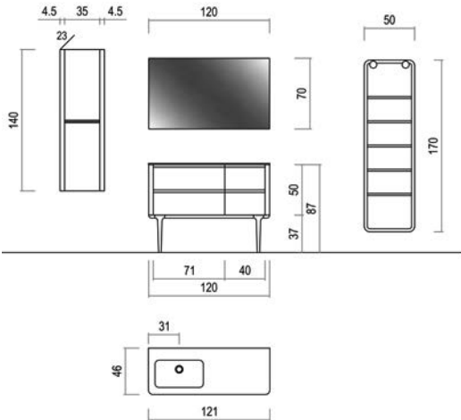
AUXILIAR VERTICAL VITE PAYNE VERTICAL AUXILIARY VITE PAYNE / AUXILIAIRE VERTICALE VITE PAYNE
