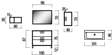
ENCIMERA TIFF TIFF COUNTERTOP / PLAN VASQUE TIFF
