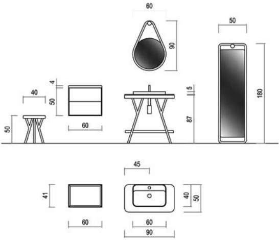
TAPA MINERALMARMO®. ESQUINAS CURVAS MINERALMARMO® COVER. CURVED CORNERS PLATEAU MINERALMARMO®. COINS ARRONDIS
